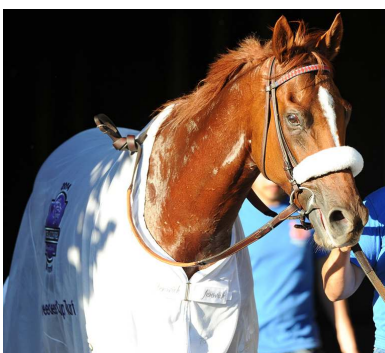
Main Sequence | A Coglianese
